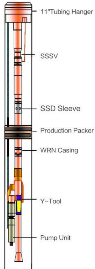
▲ 完井工具管柱/Completion Tools String
